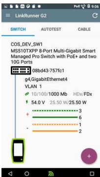
Switch Information
