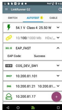
802.1x Results
