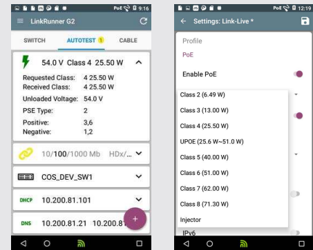
PoE Test
