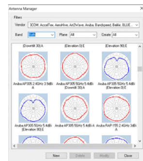
Customized Antenna Patterns
