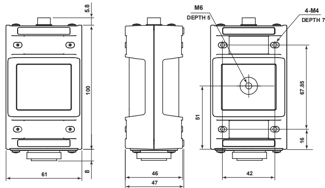
AQ2200-232 / -242 Optical Sensor Head
