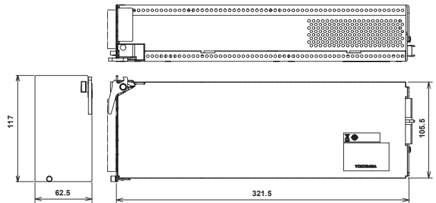
AQ2200 Series 2-Slot Size Module
