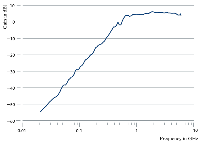
Measured realized gain of the R&S®HE400UWB
