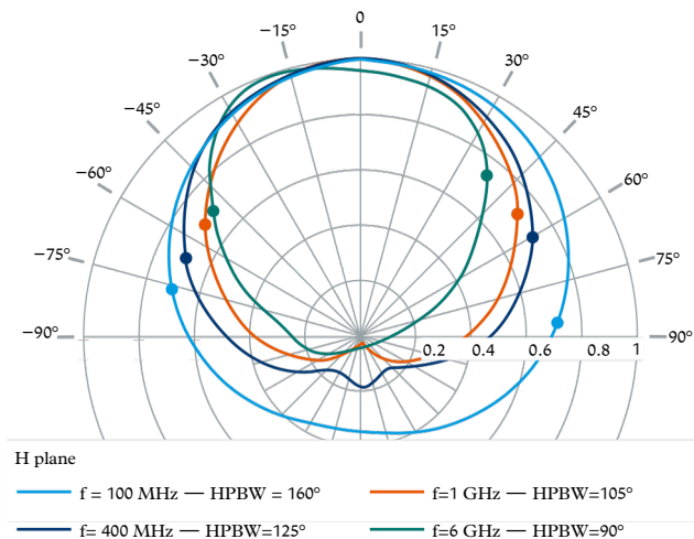
Meas. field patterns of the R&S®HE400UWB in the H plane
